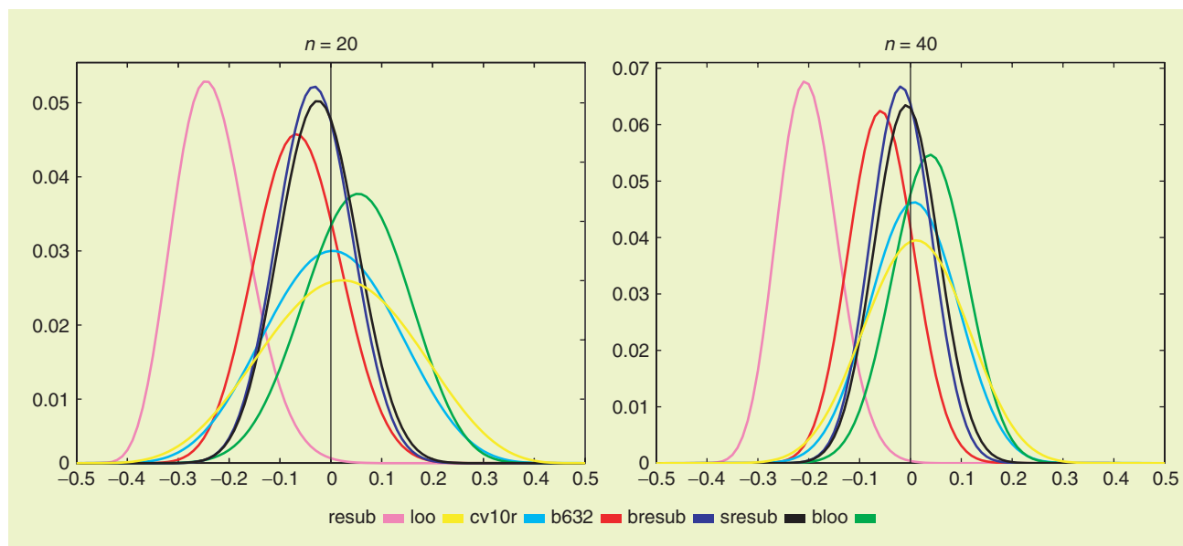
[FIG13] Beta-fit deviation distributions for CART with sample sizes n = 20 and n = 40 .
